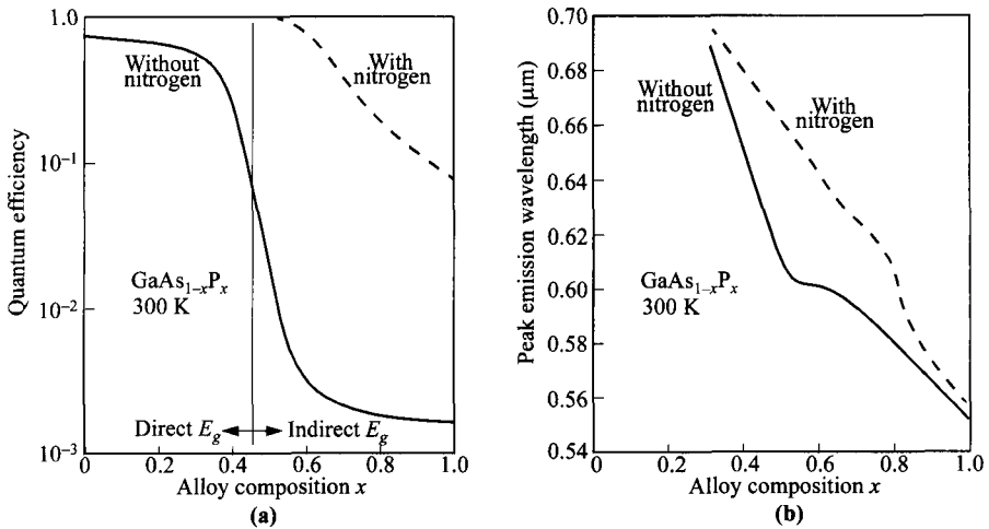
Fig. 12 (a) Quantum efficiency of \text{GaAs}_{1-x}\text{P}_x vs. alloy composition, with and without isoelectronic impurity nitrogen. (b) Peak emission wavelength vs. composition. (After Ref. 22.)
