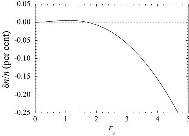
Fig. 5.8. Violation of the particle-number sum rule for the homogeneous electron gas in the G_0W_0 approximation. The relative error in the density is always negative and of the order of 0.1% in the range of metallic densities. After Schindlmayr et al. [105]
